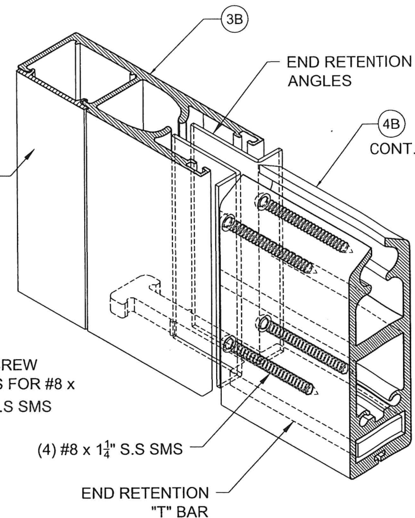
BOTTOM BAR ASSEMBLY ISOMETRIC (COMPONENT 1 NOT SHOWN FOR CLARITY)
