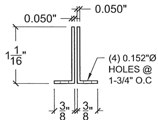
END RETENTION ANGLES (LENGTH 2 3/4") 3105-H14 ALUM. ALLOY
