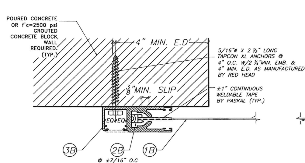
SECTION B-B: WALL MOUNTED (PLAN)* SCALE: N.T.S.
