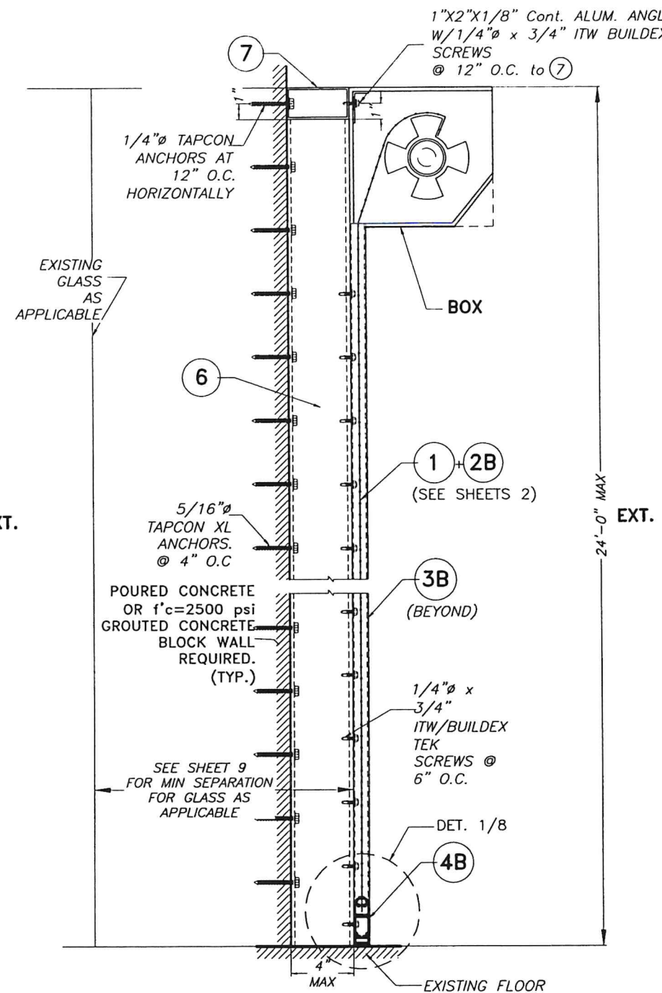
SECTION E-E BUILD OUT MOUNTED
