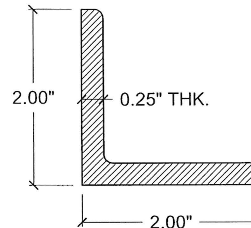
(5) TRAPPED ANGLE 6061-T6 ALUM. ALLOY
