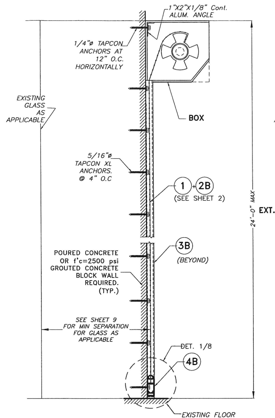
SECTION A-A WALL MOUNTED
