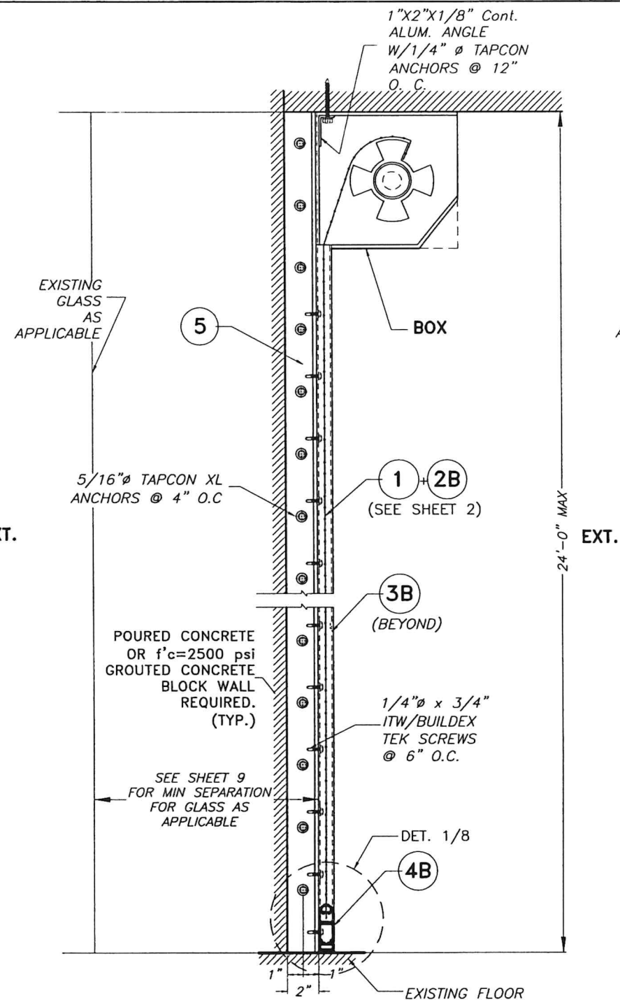
SECTION C-C TRAPPED MOUNTED
