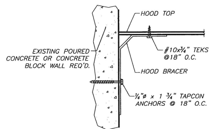
WALL HOOD ATTACHMENT (SIDE VIEW)
