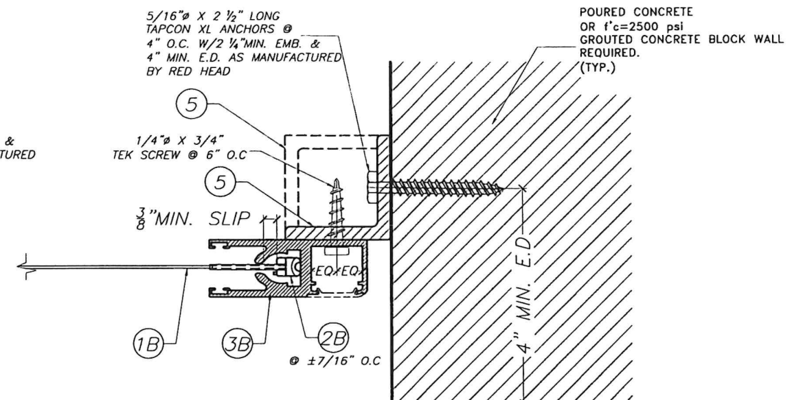
SECTION D-D: TRAPPED MOUNTED (PLAN)* SCALE: N.T.S.
