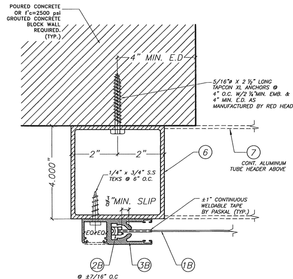
SECTION F-F: BUILD-OUT MOUNTED (PLAN)* SCALE: N.T.S.
