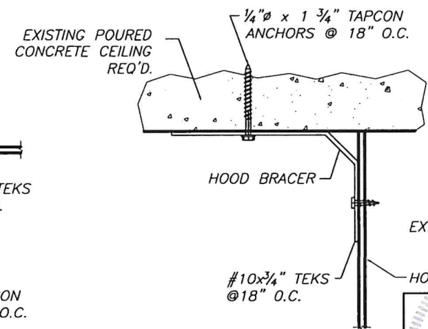
CEILING HOOD ATTACHMENT (SIDE VIEW)
